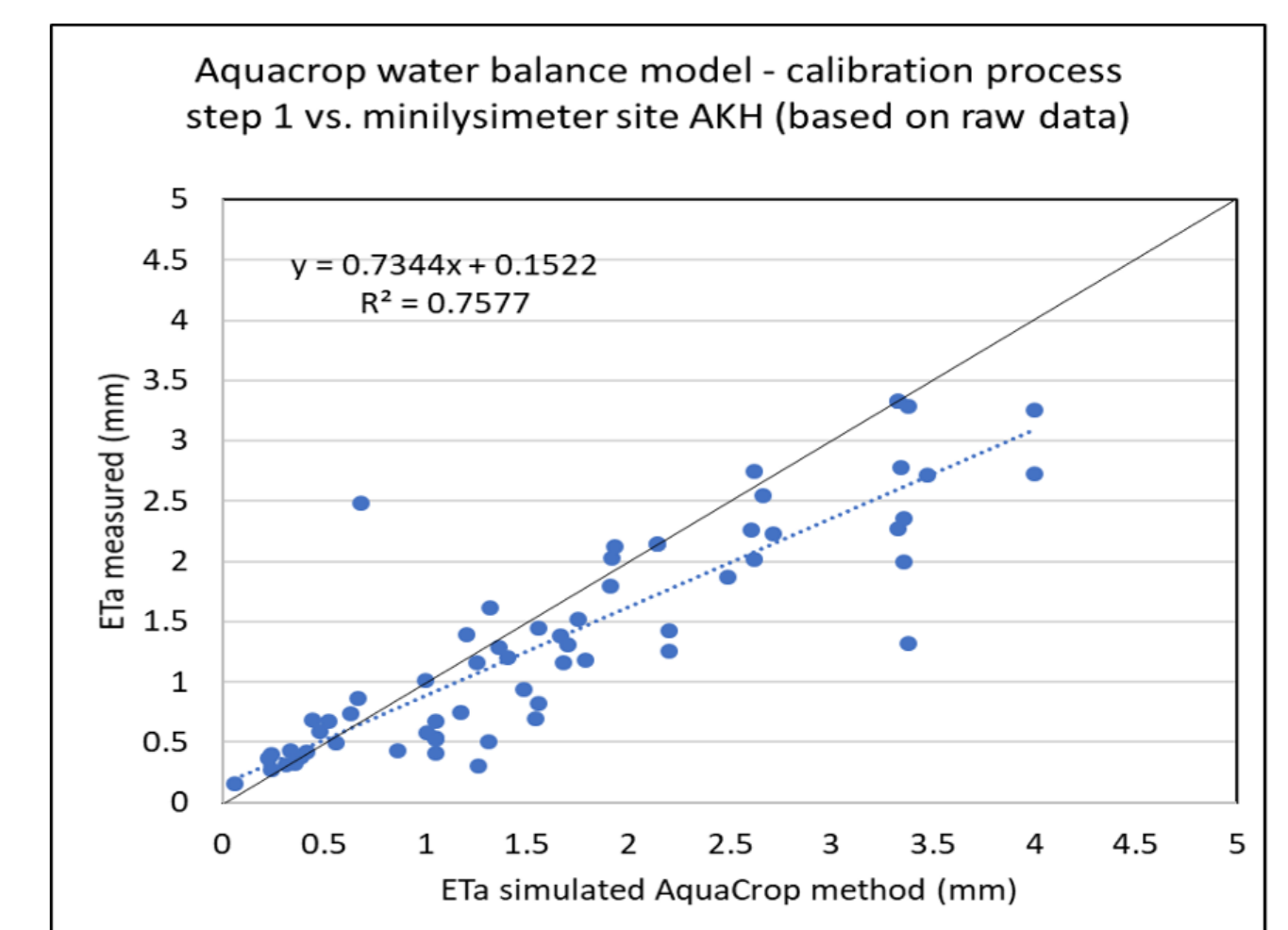
Fig. 3: Comparison of 3-day average actual evapotranspiration measured by mini lysimeter vs. simulated by Aquacrop method (uncalibrated)
