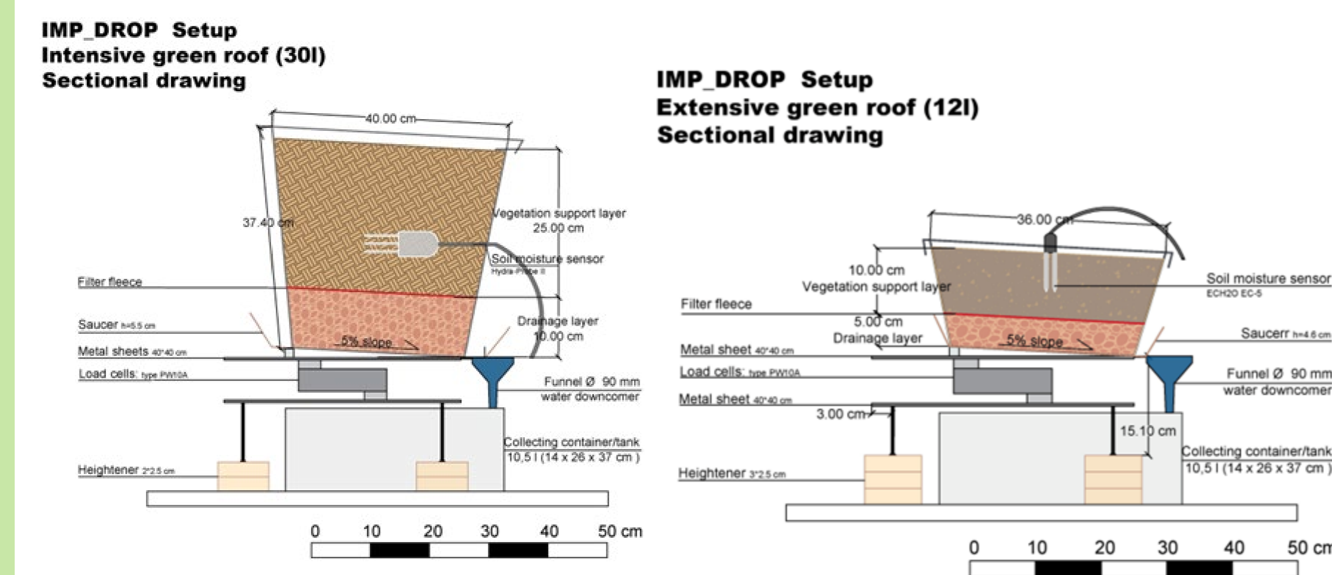
Figure 2: Sectional drawing of the experimental setup of the lysimeter for the investigation of an intensive (left) and extensive (right) green roof
